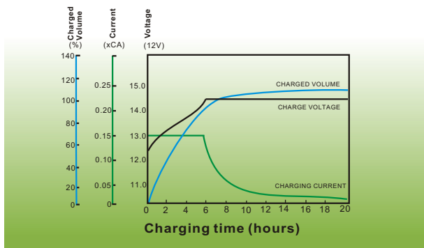
Constant voltage charging characteristic (0.15CA, 25°C, 77°F)
